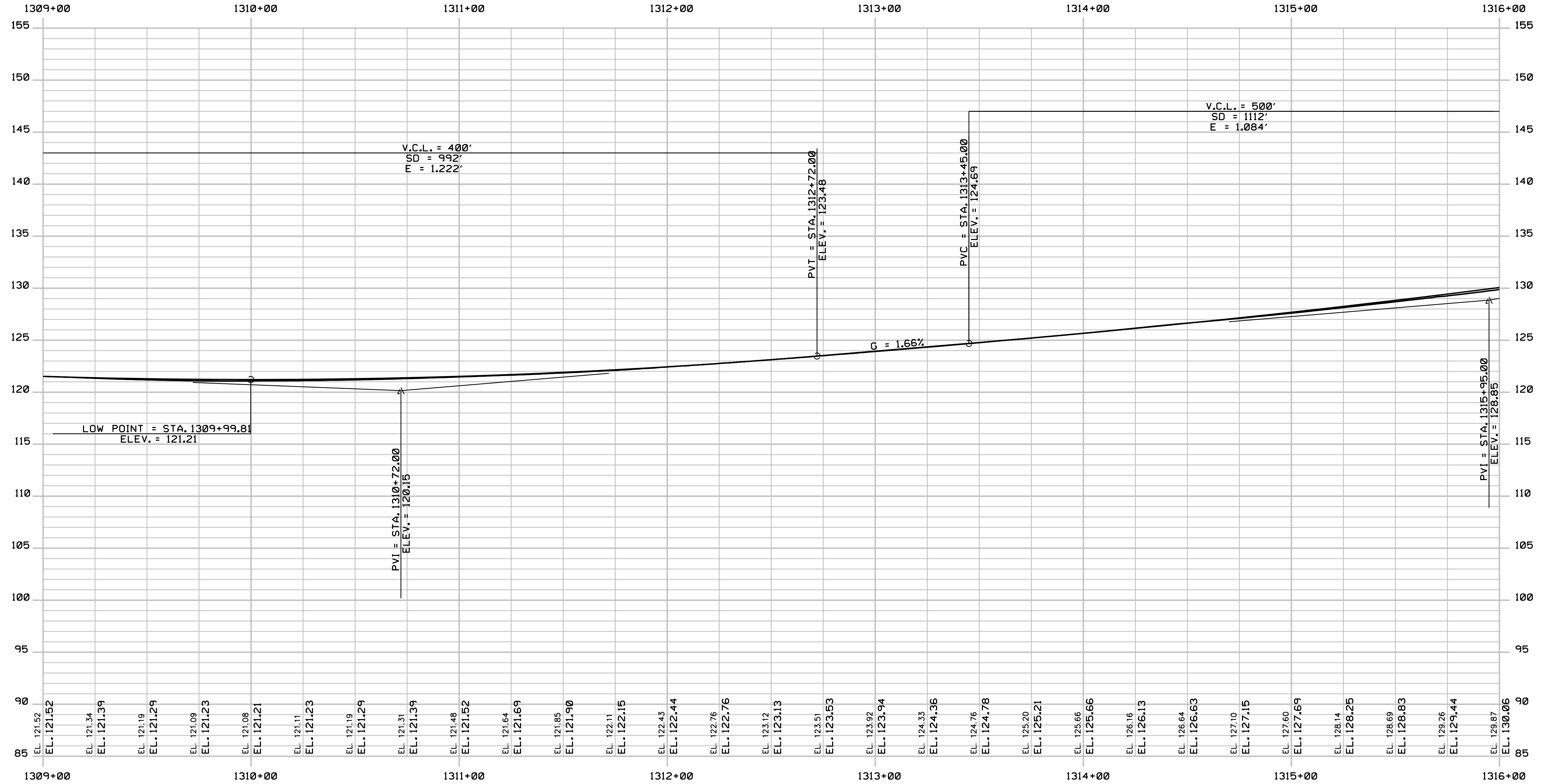
PROFILE
