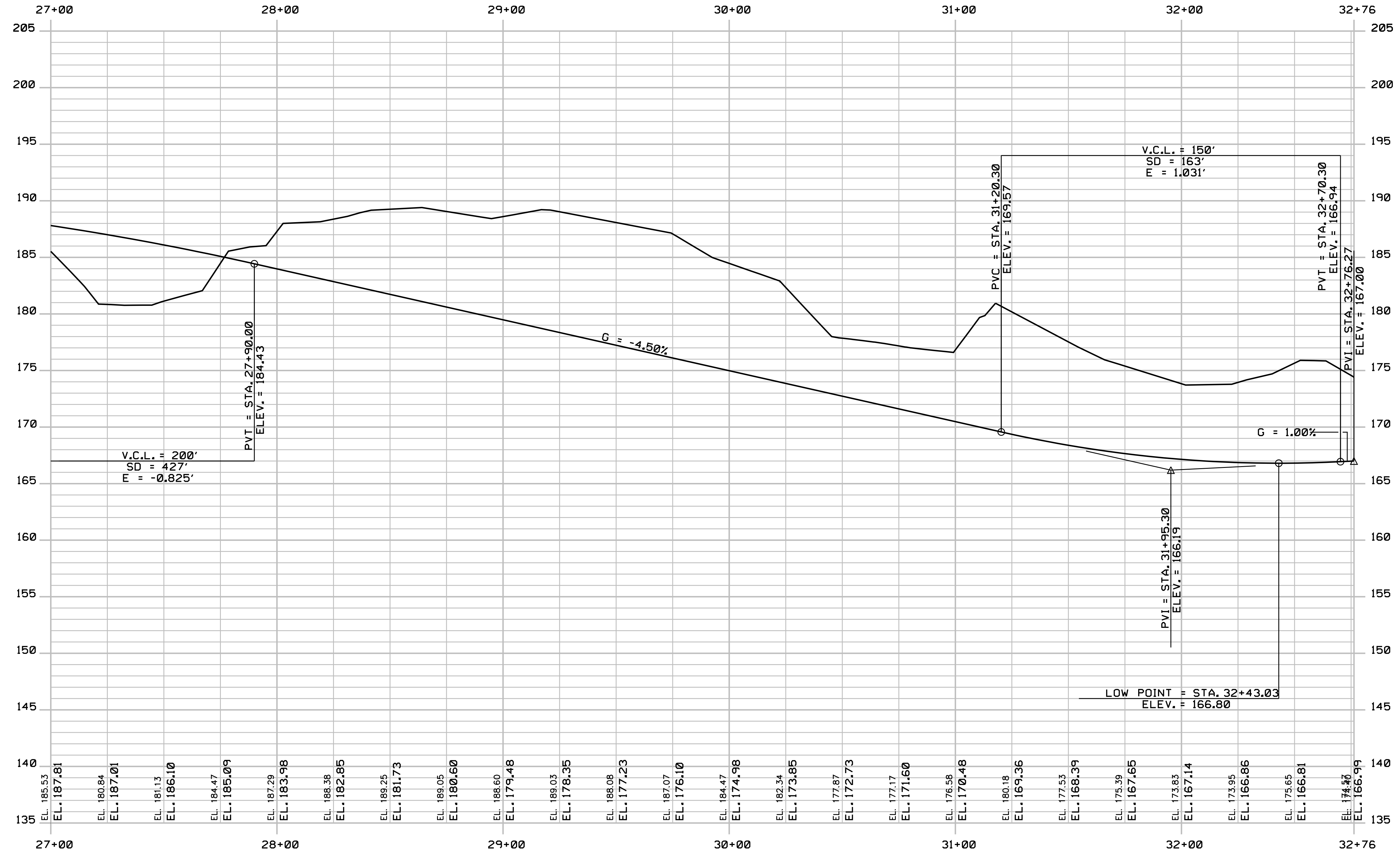
PROFILE
